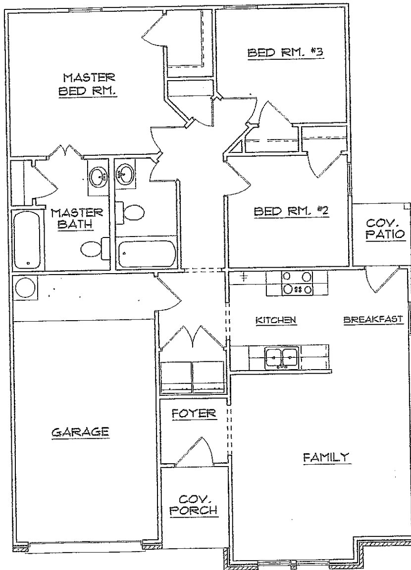
"THE LADIN" 1052 SQ. FT. LIVING AREA
